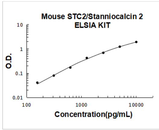
Mouse STC2 PicoKine ELISA Kit Standard Curve
