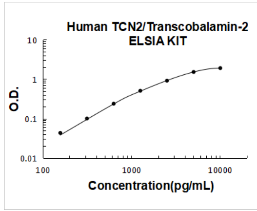
Human TCN2 PicoKine ELISA Kit Standard Curve
