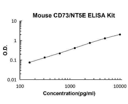
Mouse NT5E PicoKine ELISA Kit standard curve
