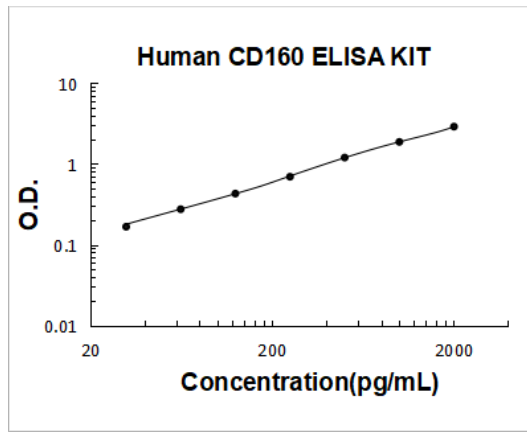
Human CD160 PicoKine ELISA Kit Standard Curve
