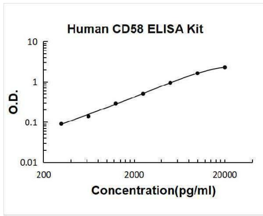
Human CD58 PicoKine ELISA Kit standard curve
