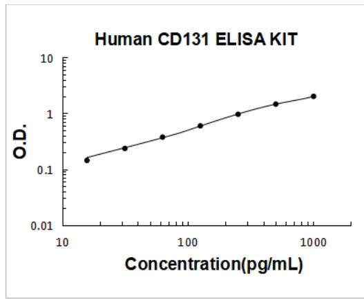
Human CD131 PicoKine ELISA Kit standard curve
