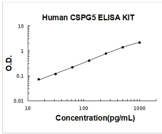
Human CSPG5 PicoKine ELISA Kit standard curve
