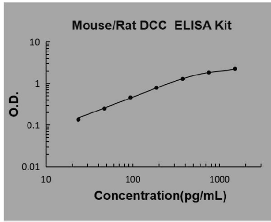
Mouse/Rat DCC PicoKine ELISA Kit standard curve
