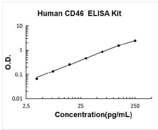
Human CD46 PicoKine ELISA Kit standard curve
