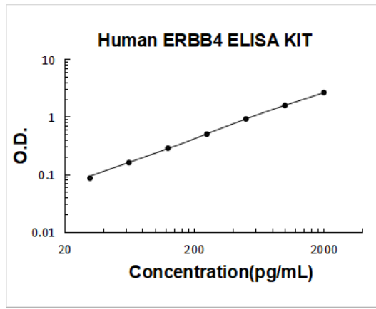
Human ERBB4 PicoKine ELISA Kit standard curve
