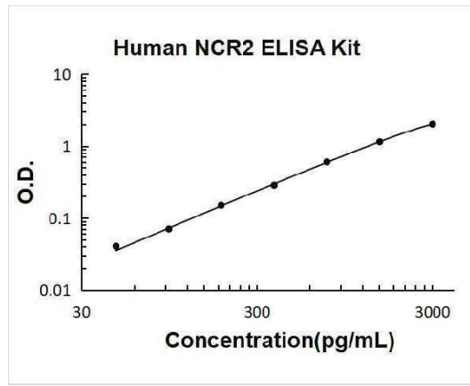
Human NCR2 PicoKine ELISA Kit standard curve
