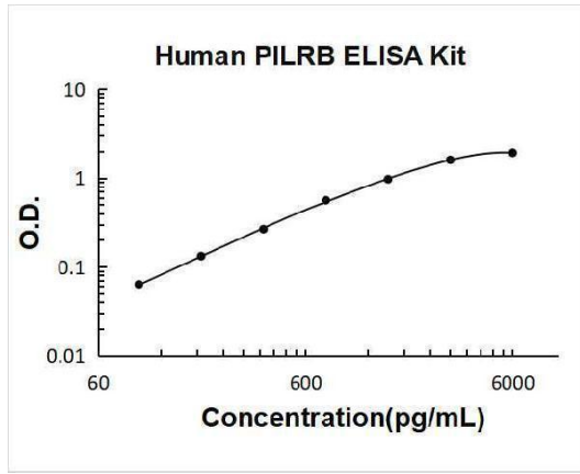
Human PRLRB PicoKine ELISA Kit standard curve
