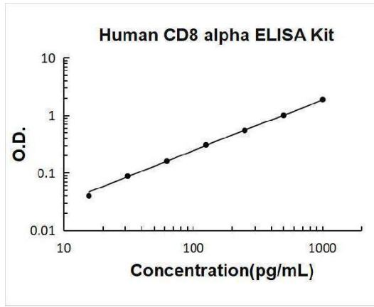
Human CD8 alpha PicoKine ELISA Kit standard curve
