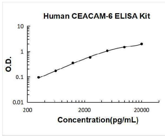
Human CEACAM-6 PicoKine ELISA Kit standard curve
