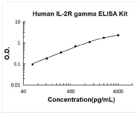
Human IL-2R gamma PicoKine ELISA Kit standard curve
