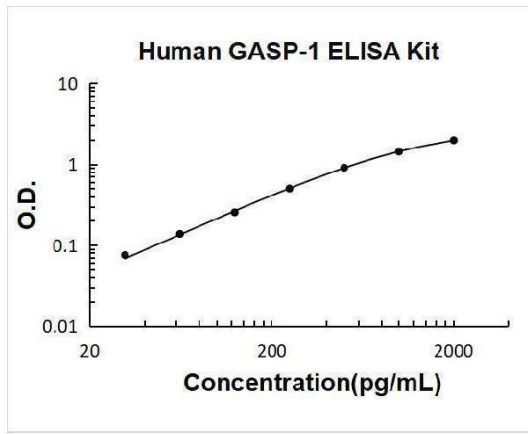
Human GASP-1 PicoKine ELISA Kit standard curve
