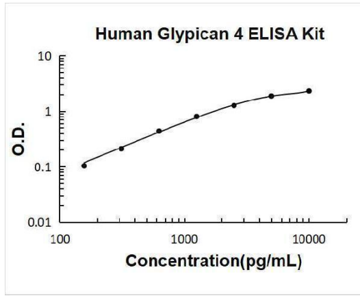
Human Glypican 4 PicoKine ELISA Kit standard curve
