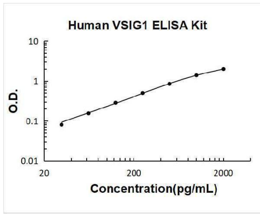
Human VSIG1 PicoKine ELISA Kit standard curve
