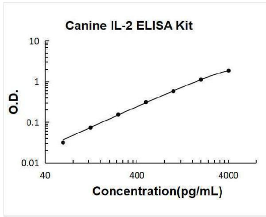
Canine IL-2 PicoKine ELISA Kit standard curve
