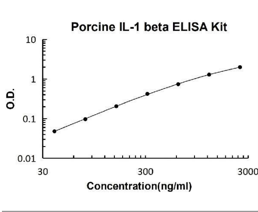
Porcine IL-1 beta PicoKine ELISA Kit standard curve
