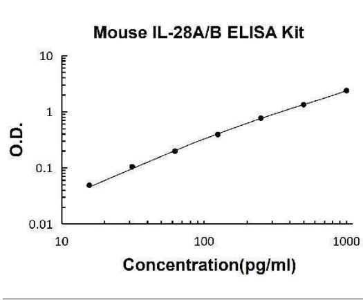
Mouse IL-28A/B PicoKine ELISA Kit standard curve
