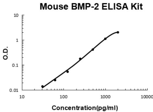
Mouse BMP-2 PicoKine ELISA Kit standard curve
