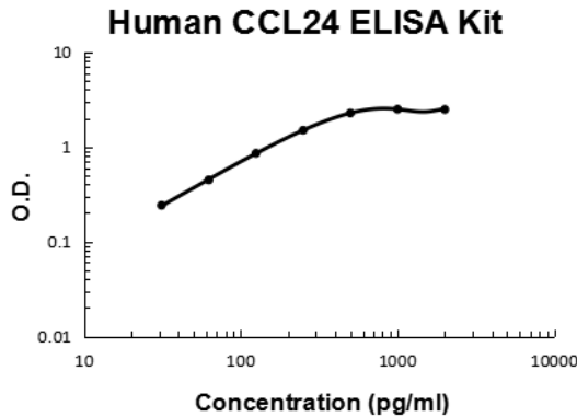
Human CCL24 PicoKine ELISA Kit standard curve
