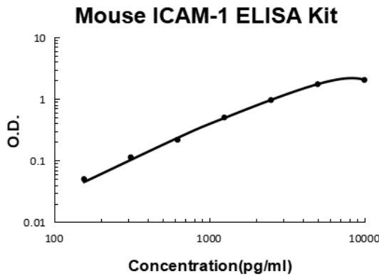
Mouse ICAM-1 PicoKine ELISA Kit standard curve
