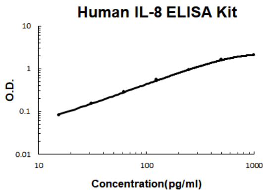
Human IL-8 PicoKine ELISA Kit standard curve
