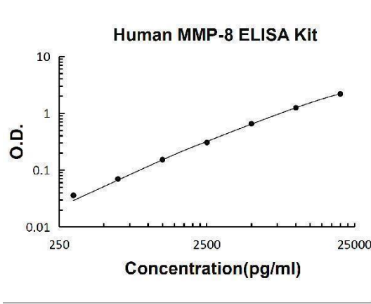
Human MMP-8 PicoKine ELISA Kit standard curve
