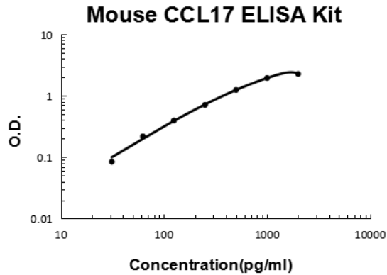
Mouse CCL17 PicoKine ELISA Kit standard curve
