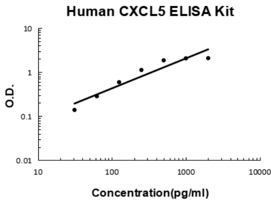
Human CXCL5/ENA-78 PicoKine Quick ELISA Kit standard curve
