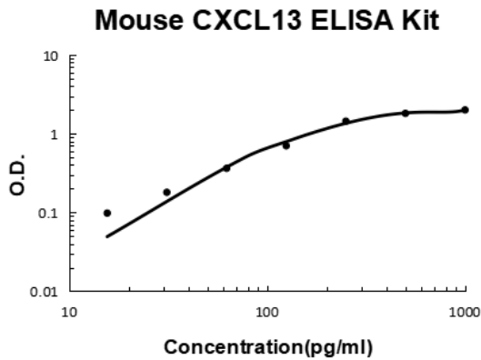
Mouse CXCL13/BLC PicoKine ELISA Kit standard curve
