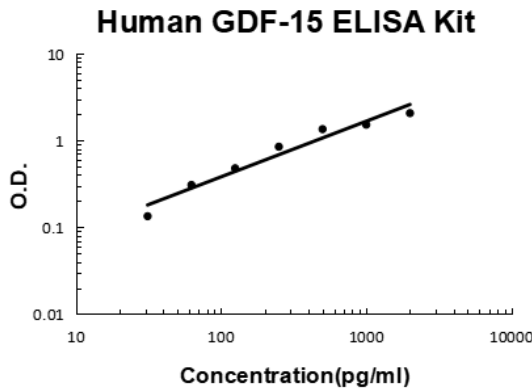
Human GDF-15 PicoKine ELISA Kit standard curve
