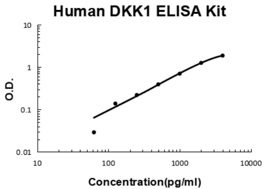
Human DKK1 PicoKine ELISA Kit standard curve
