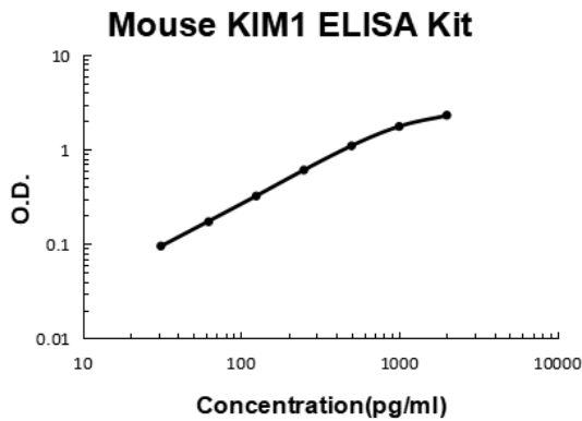
Mouse KIM1 PicoKine ELISA Kit standard curve
