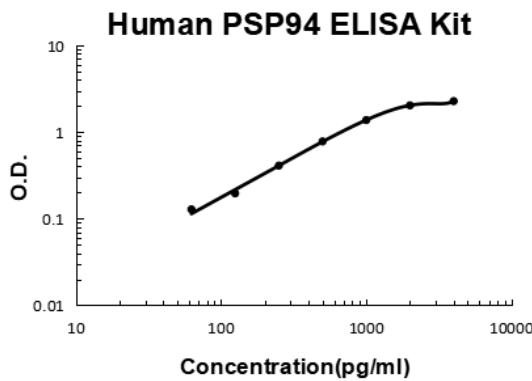
Human PSP94 PicoKine ELISA Kit standard curve
