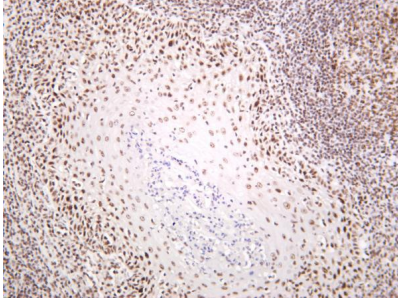
Human tonsil was stained with anti-Nucleolin rabbit antibody
