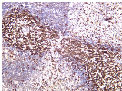
Mouse spleen was stained with anti-CD3 rabbit antibody
