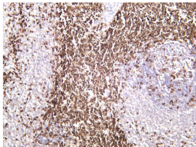
Rat spleen was stained with anti-CD3 rabbit antibody
