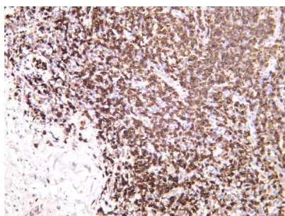
Human tonsil was stained with anti-CD3 rabbit antibody
