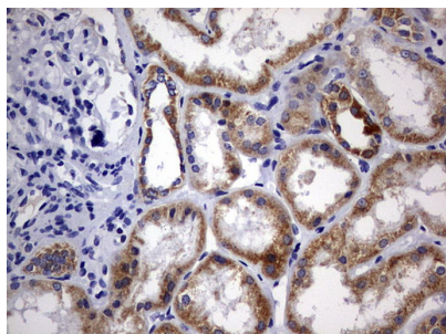
Immunohistochemical staining of paraffin-embedded Human Kidney tissue within the normal limits using anti-DAP3 mouse monoclonal antibody. (Heat-induced epitope retrieval by 10mM citric buffer)
