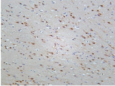
Human brain was stained with Anti-TBR1 rabbit antibody
