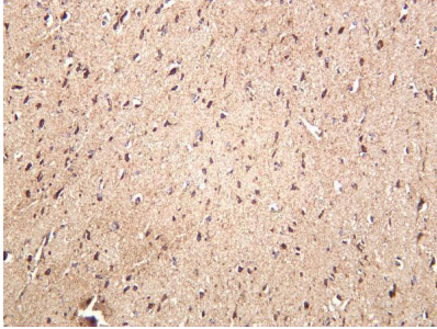
Human brain was stained with anti-NDUFB8 rabbit antibody
