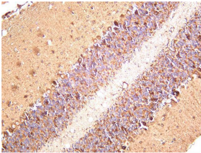
Mouse brain was stained with anti-NDUFB8 rabbit antibody
