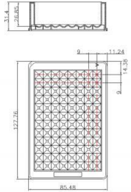
96 Channel Troughs, Single Well, middle Profile
