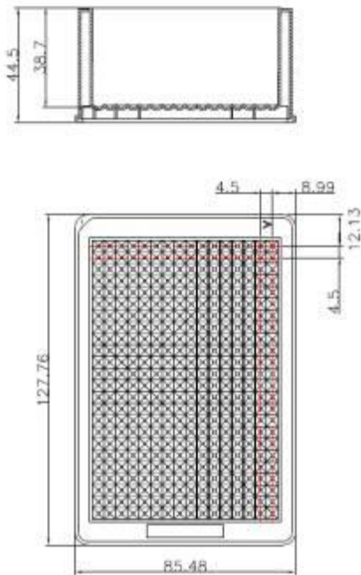
384 Channel Troughs, Single Well, High Profile
