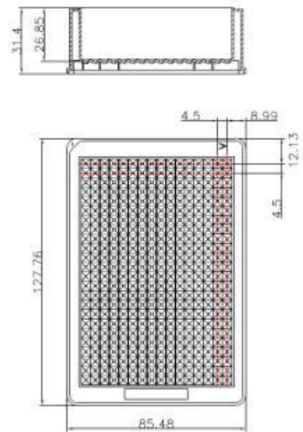
384 Channel Troughs, Single Well, middle Profile
