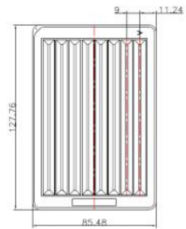
8 Channel Troughs, Multi Well, middle Profile
