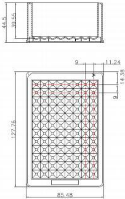
96 Channel Troughs, Single Well, High Profile
